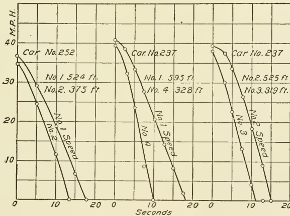
Fig. 130. Acceleration Curves
